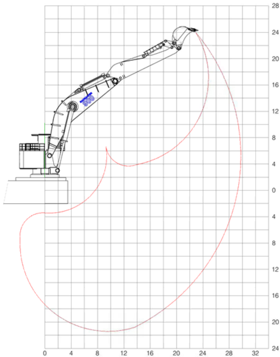
Dredging Diagram
